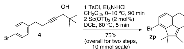
Scheme 4. C–H functionalization of ω-aryl-substituted propargylic alcohol derivatives: tosylation and double arylation reactions.
